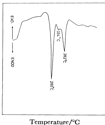
Fig. 9. DTA thermogram of hexaamminecobalt(III) hexachloroferrate(III) in air.
